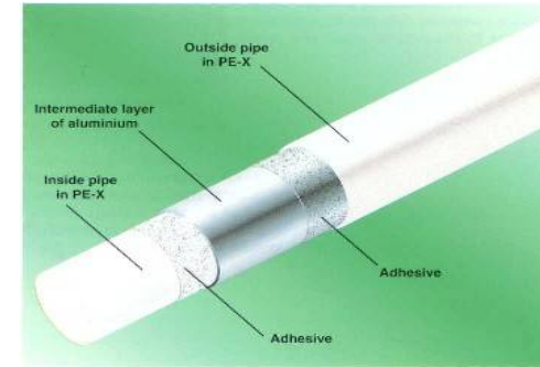
Multi-layer tubing
